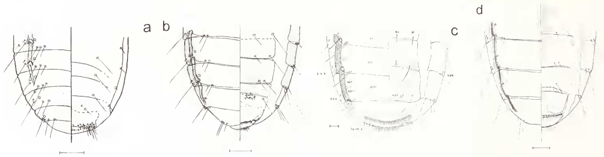
Fig. 5. Abdominal segments and the terminal plates of a: Trochiloecetes ochoterena? , b: " Trochiliphagus ", c: Ricinus brevipitatis (after NELSON 1972, plate 3) and d: R. dolichocephalus (from RHEINWALD 1968, Fig. 13). Left from dorsal, right from ventral. Scale bar 0.1 mm.
